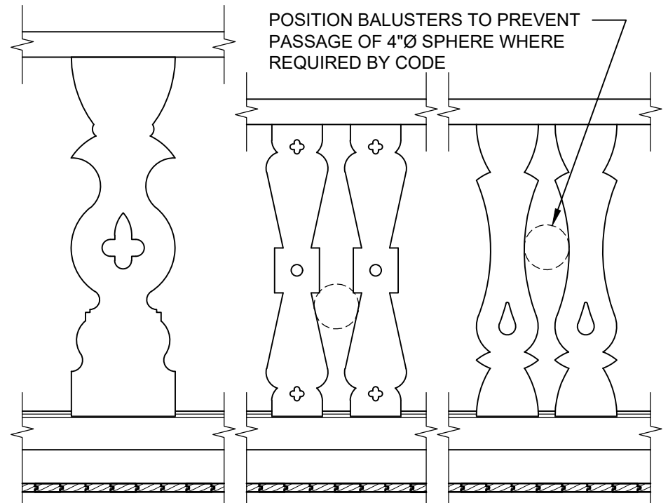
SAW-CUT BALUSTERS (DIMENSIONS AND STYLE VARIES)
