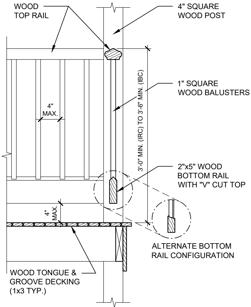
RAILING SECTION
